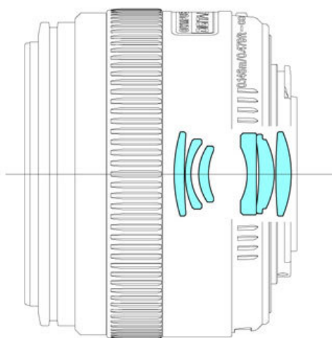
35mm Macro f3,5 ( \infty , open aperture)
