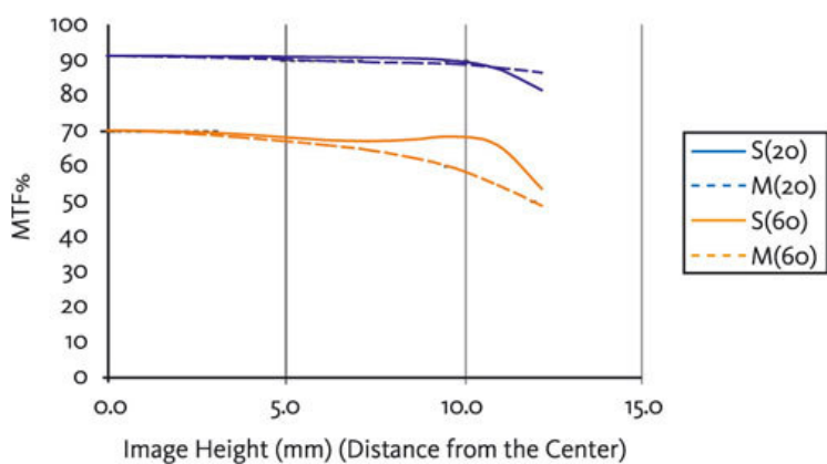
35mm Macro f3,5 ( \infty , open aperture)
